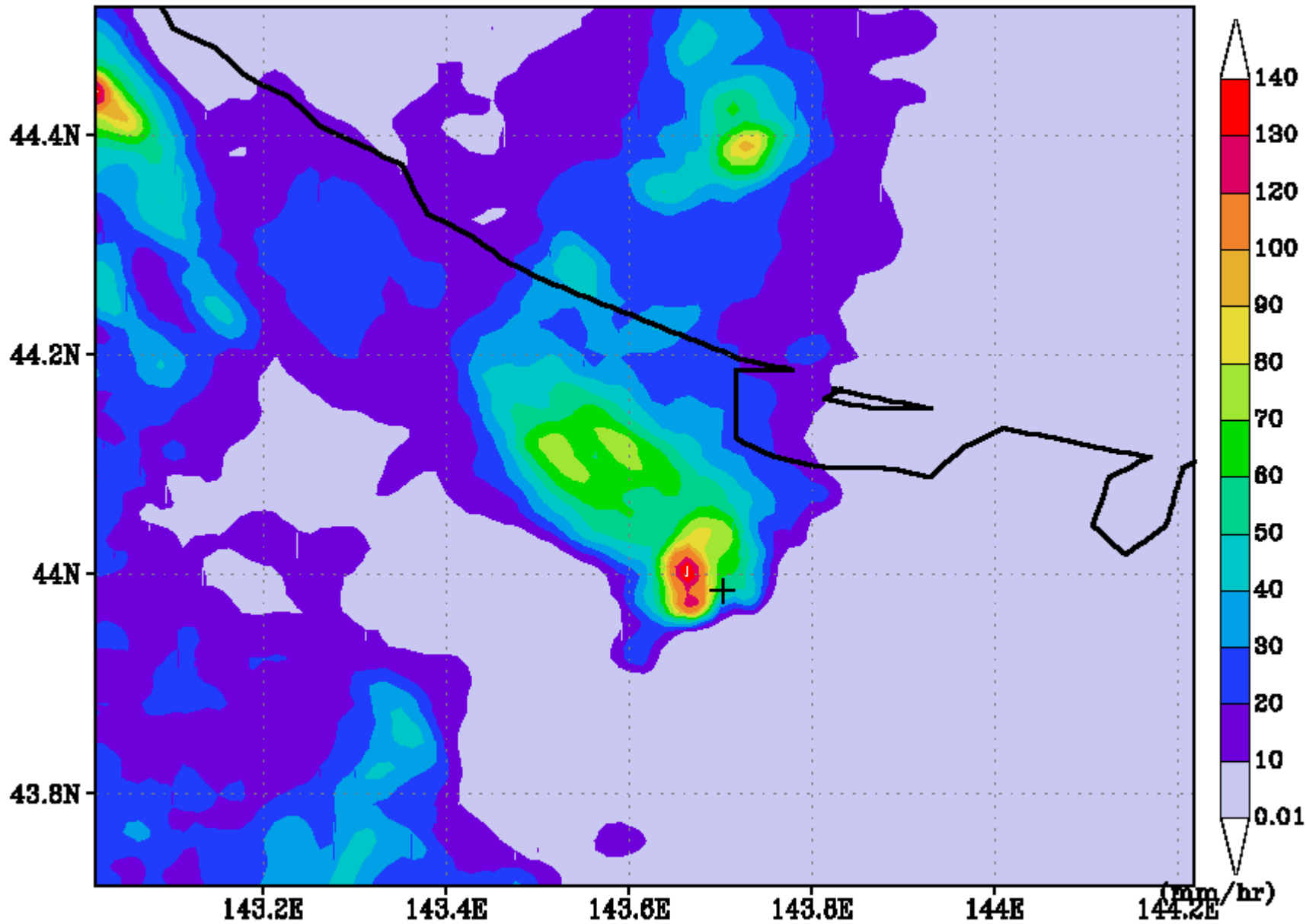
04:30Z07NOV2006: JMA radar, rainfall rate (mm/hr)
