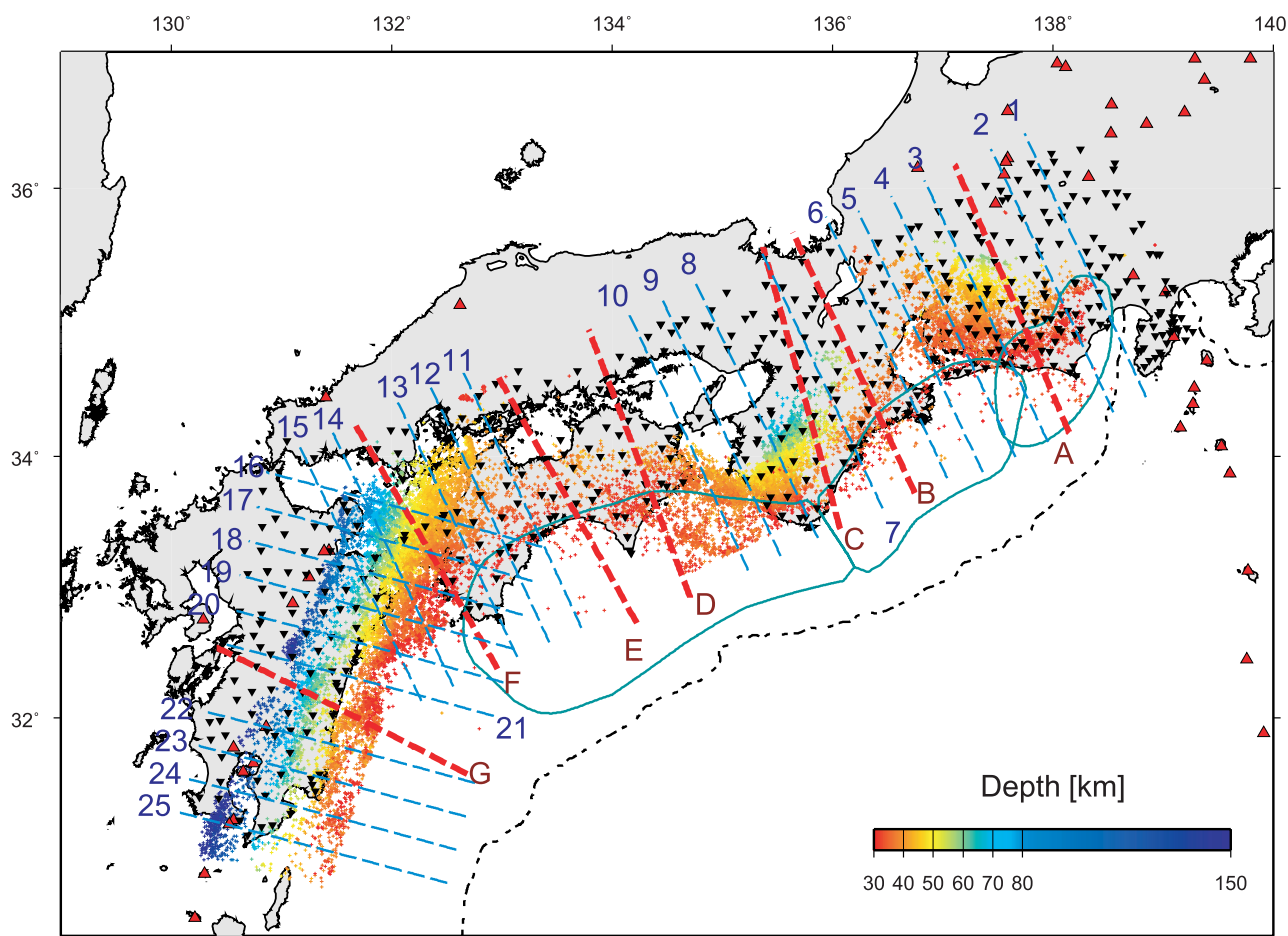
Figure 2. Epicenter distribution of earthquakes (crosses) at depths of 30–150 km and seismograph stations (solid reverse triangles) used in the double-difference tomography. Colors indicate the depth of hypocenters according to the color scale. Dashed blue lines show the locations of vertical cross sections 1 through 25 (see Figures 4–6). Dashed red lines denote the locations of vertical cross sections (A–G) for which the obtained velocity structures are compared with the results of seismic refraction surveys (Figures 7 and 9–14). Other symbols are the same as those in Figure 1.
