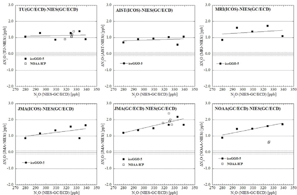
Figure 22. Differences of the measured N_2O concentration between participating laboratories and the NIES as a function of N_2O concentrations for the TU, AIST, MRI, JMA, and NOAA datasets. The solid line represents a least-squares fit to all data points from the iceGGO-5 and NOAA-ICP experiments.
