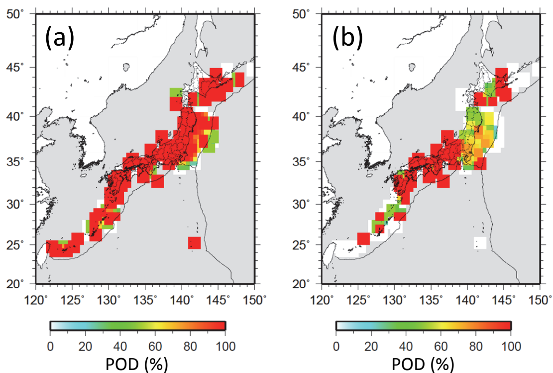
Fig. 5 Distribution of POD ( M \geq 1.0 ) in a grid of 1 \times 1 degree of (a) this study, and (b) the current system.
