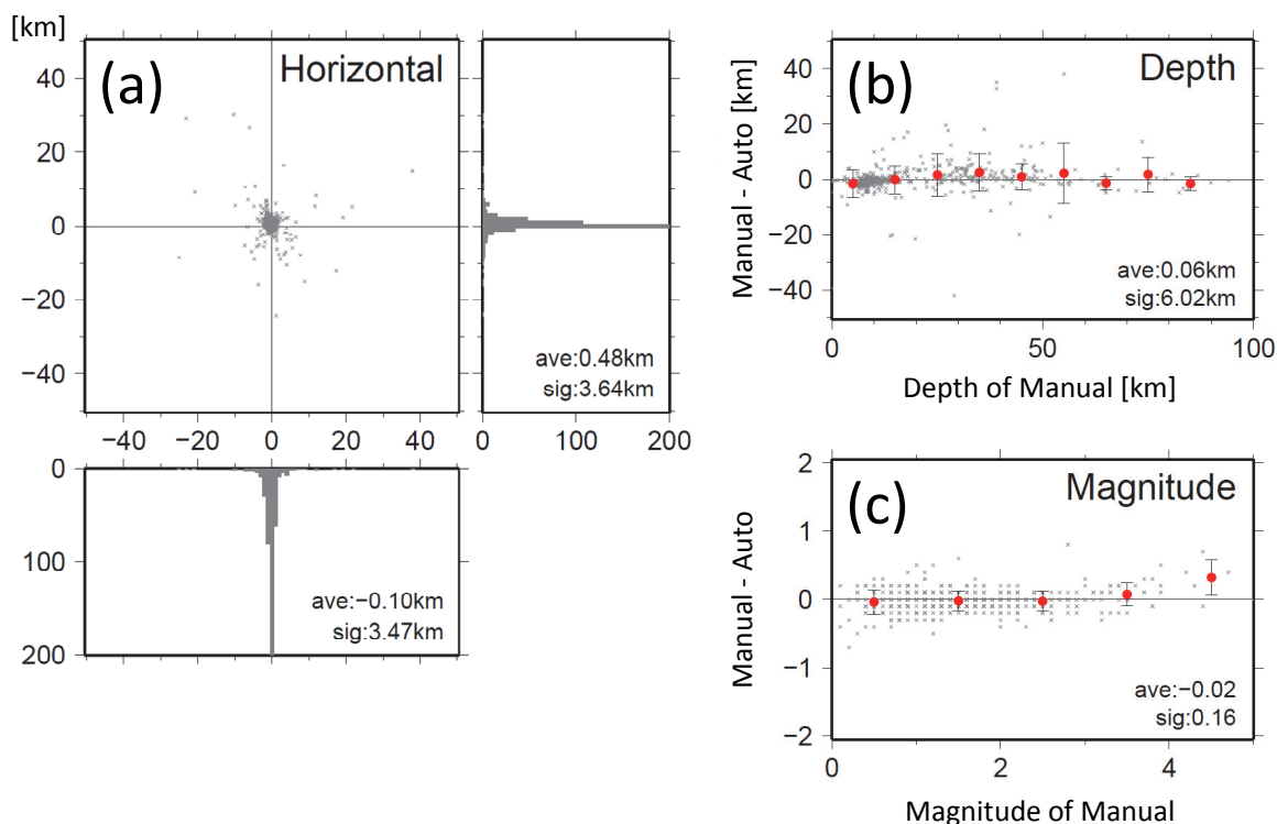
Fig. 6 (a) Distribution of residuals between manual and automatic hypocenters. Histogram shows the number of residuals per 1 km. (b) Residual of depth between manual and automatic hypocenters. Mean and error bar averaged every 10 km. (c) Residual of magnitude between manual and automatic hypocenters. Mean and error bar averaged every M1.
