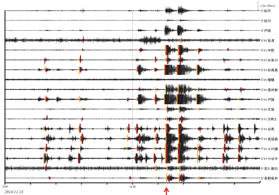
Fig. 8 Plot of seismograms of aftershocks in northern Nagano Prefecture during a 10 minute period. P- and S- wave arrival times picked by this study are shown by yellow and red bars. The current system could detect only one event in this case, which is shown by arrow at bottom.
