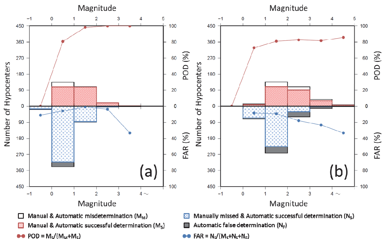
Fig. 4 Comparison of numbers of manual hypocenters and automatic hypocenters in each magnitude range. (a) Inland and shallow events ( depth \leq 30km ), (b) others such as offshore or deep events.
