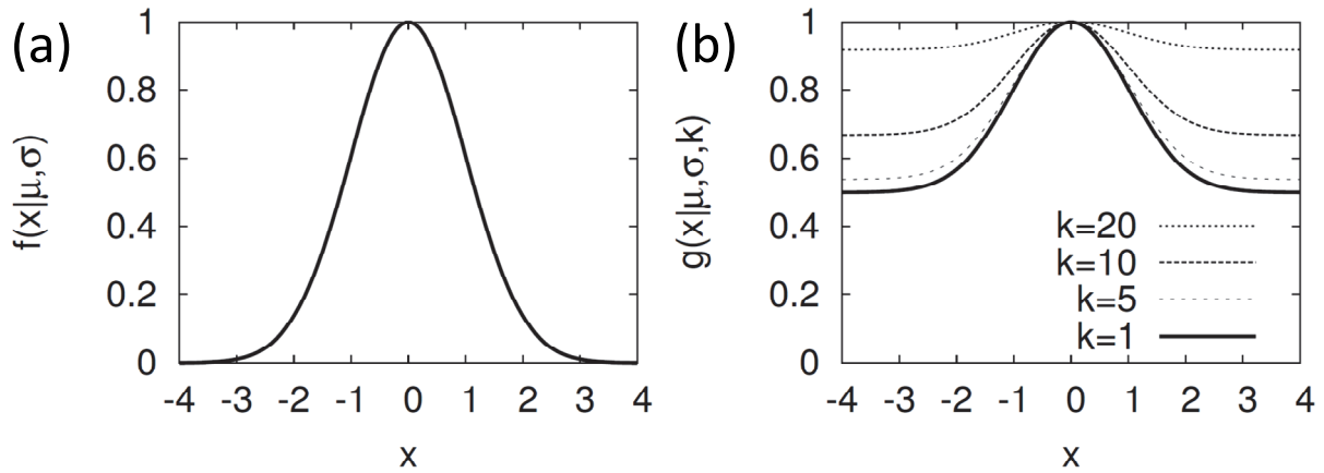
Fig. 2 (a) Normal distribution in Eq. 6. (b) Probability density function g with \mu=0 and \sigma=1 in Eq. 7. It is normal distribution with the lower bound of g_0 .
