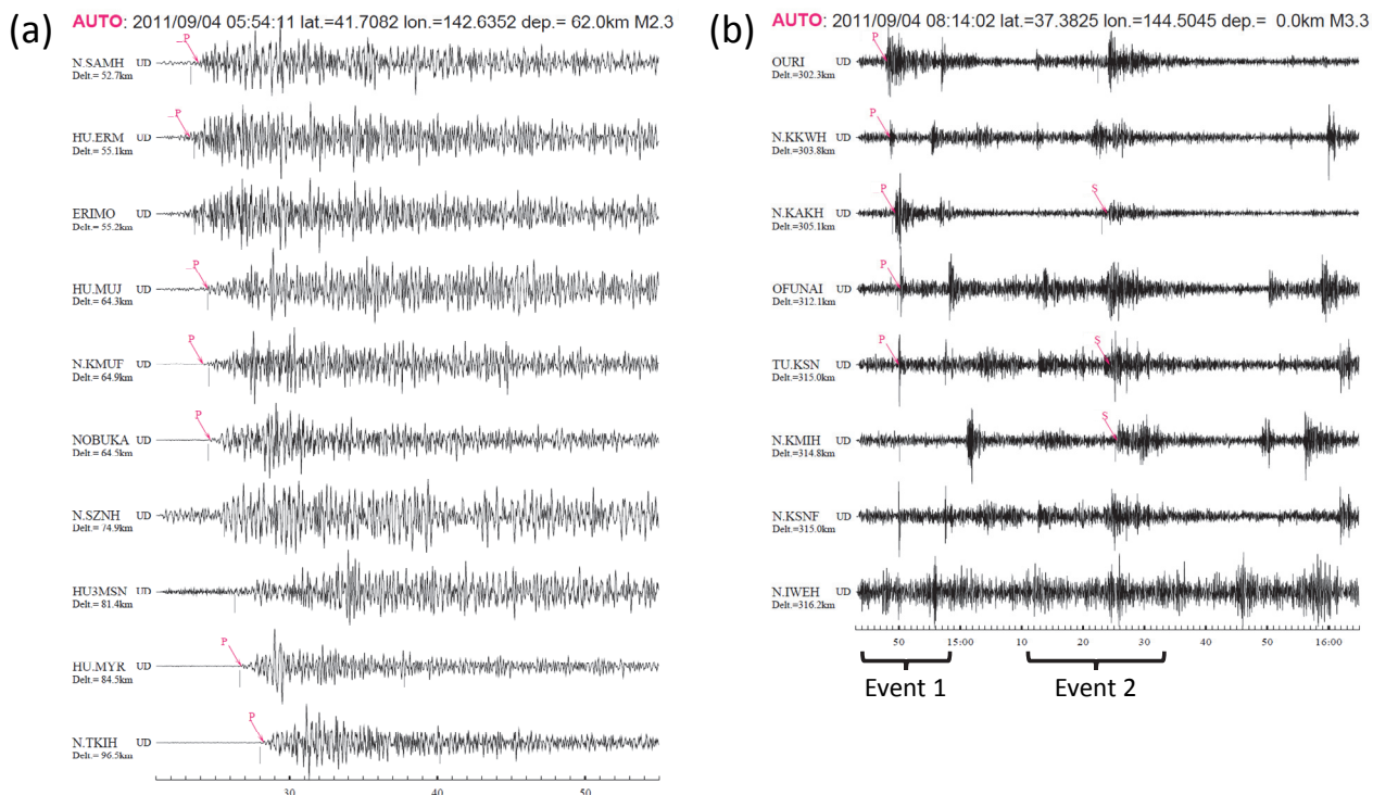
Fig. 7 Examples of false determination. (a) An earthquake occurred at Eastern Saitama Prefecture (89km depth, M4.7), but the method in this study made a false determination off Urakawa. (b) False determination of multiple earthquakes off Fukushima Prefecture (M1.5, Event 1) and off Miyagi Prefecture (M undefined, Event 2). Each seismogram shows band-pass-filtered (5-10 Hz) UD-component.
