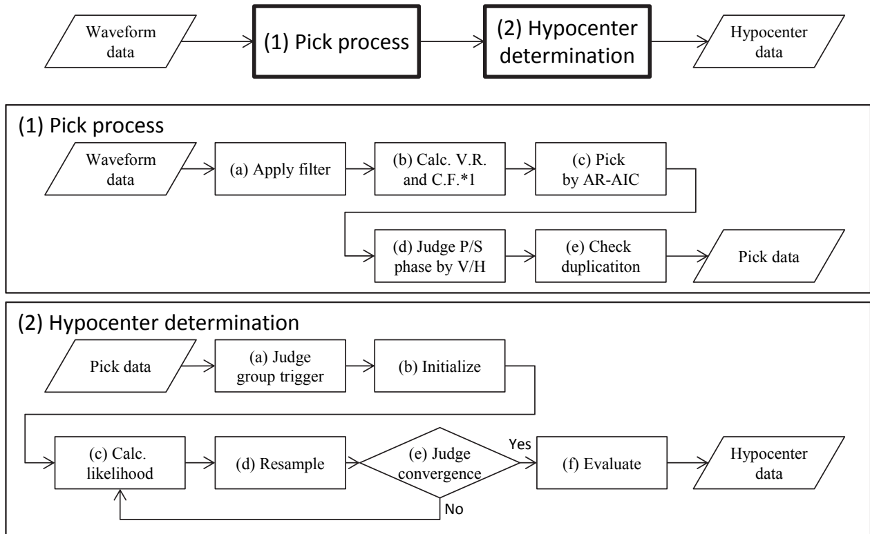
Fig. 1 Flow of automatic process. *1: V.R. means variance ratio in Eq. 1. C.F. means characteristic function in Eq. 2.
