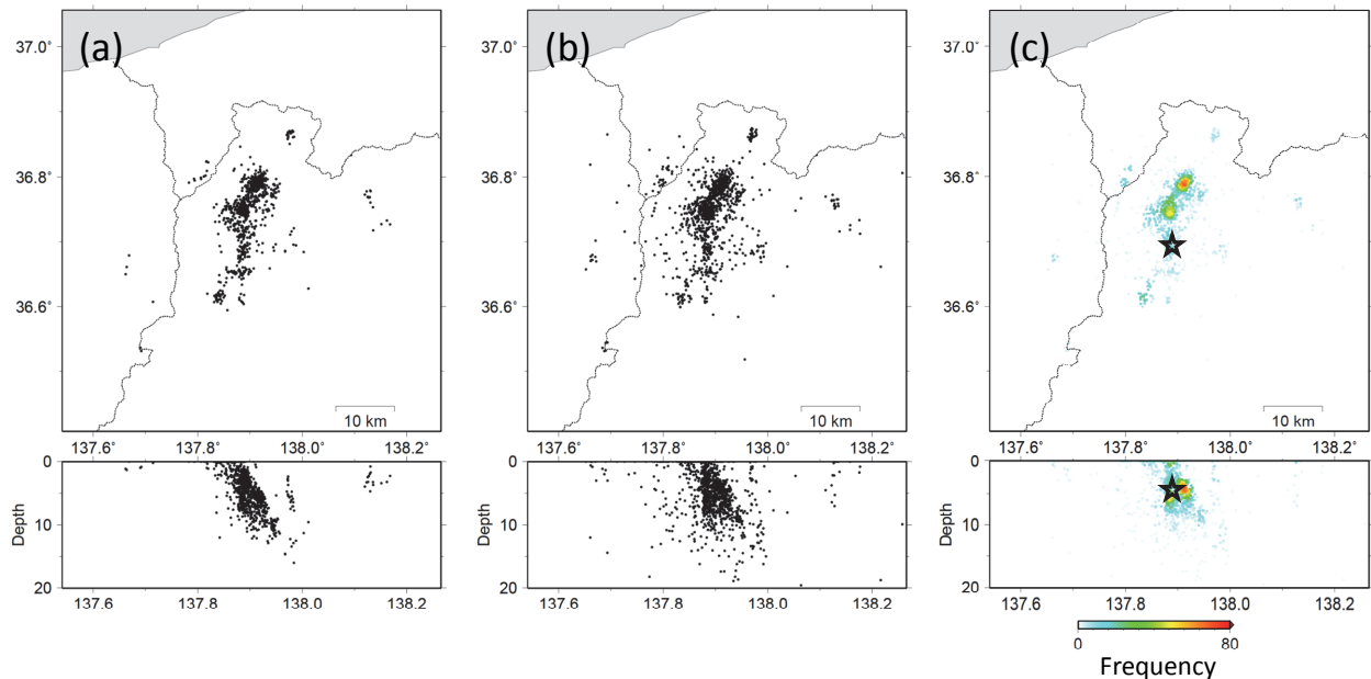
Fig. 9 Hypocentral distribution of the earthquakes ( M>0.5 ) in northern Nagano Prefecture for the period of 24 hours after the main shock on November 22, 2014 ( M6.8 ). (a) Manual hypocenters, (b) automatic hypocenters detected by this study, and (c) frequency distribution of automatic hypocenters detected in this study. Frequency distribution shows a number of hypocenter within a radius of 1 km on each plot. A star shows the manually-located main shock.
