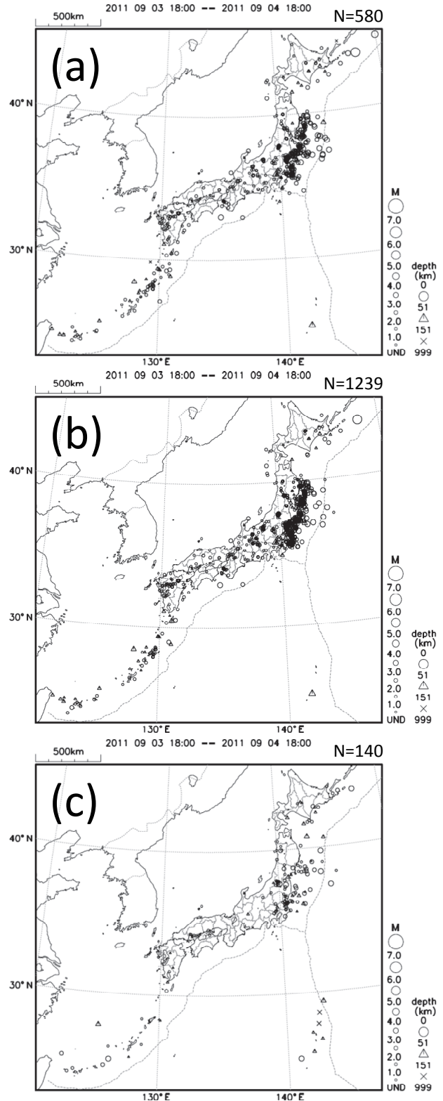
Fig. 3 Hypocentral distribution around Japan during 24 hours from 18:00 on September 3, 2011. (a) Manually checked hypocenters, (b) successful determination of automatic hypocenters in this study, (c) false determination of automatic hypocenters in this study.
