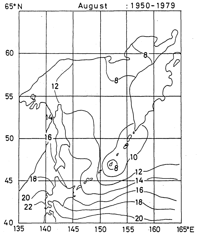
Fig. 5. 4 Monthly mean sea surface temperature (°C) (July-August)
