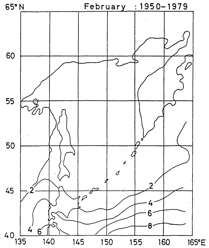
Fig. 5.1 Monthly mean sea surface temperature (°C) (January-February)
