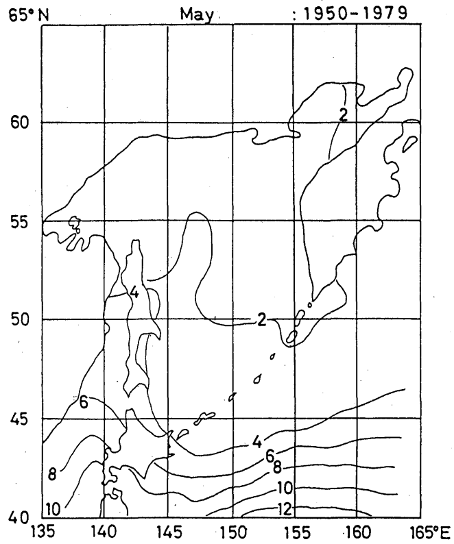
Fig. 5. 3 Monthly mean sea surface temperature (°C) (May-June)
