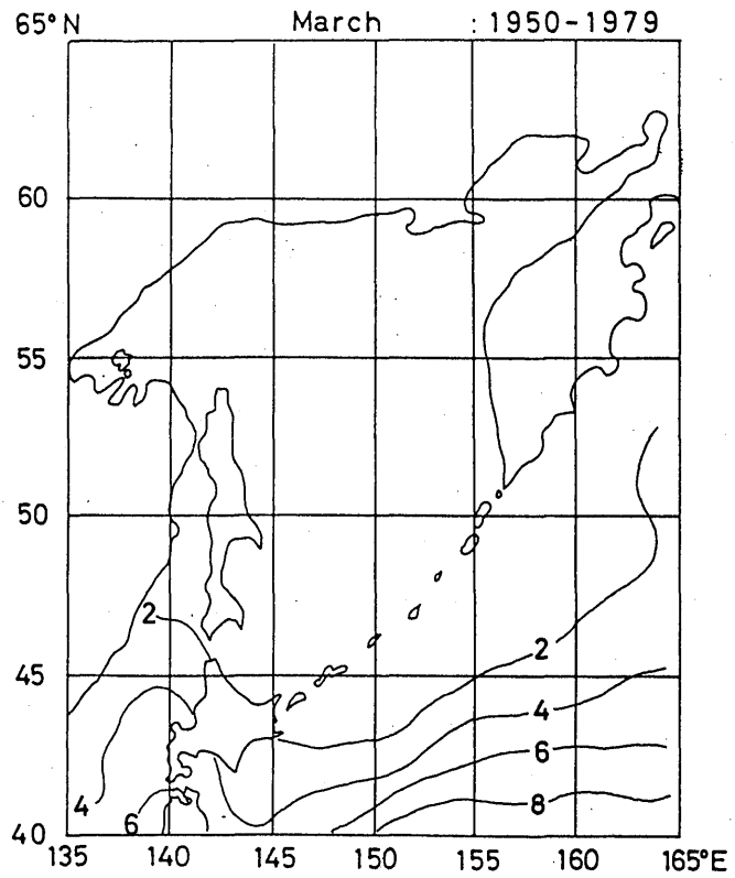
Fig. 5. 2 Monthly mean sea surface temperature (°C) (March-April)
