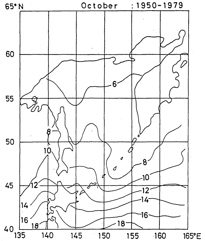
Fig. 5.5 Monthly mean sea surface temperature (°C) (September–October)
