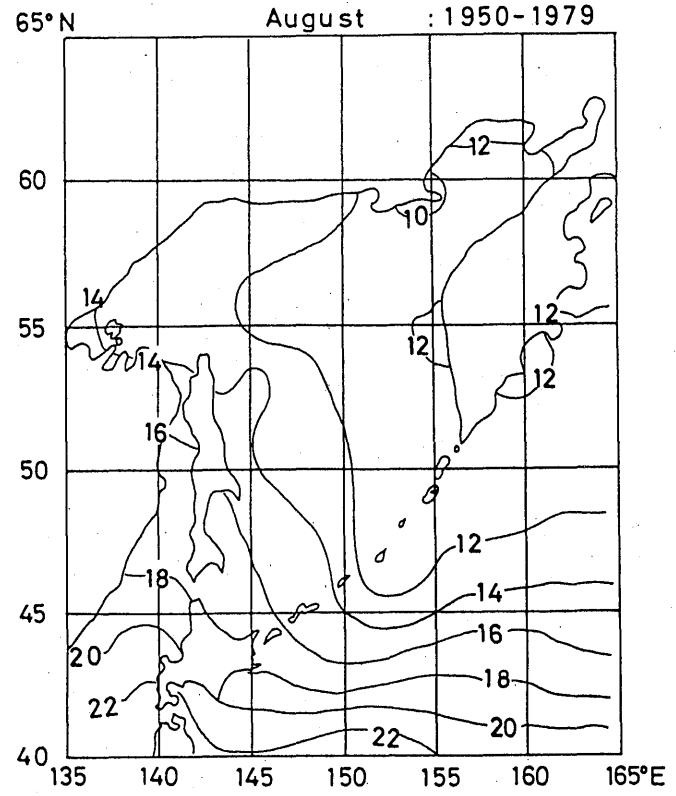
Fig. 4. 4 Monthly mean surface air temperature (°C) (July-August)
