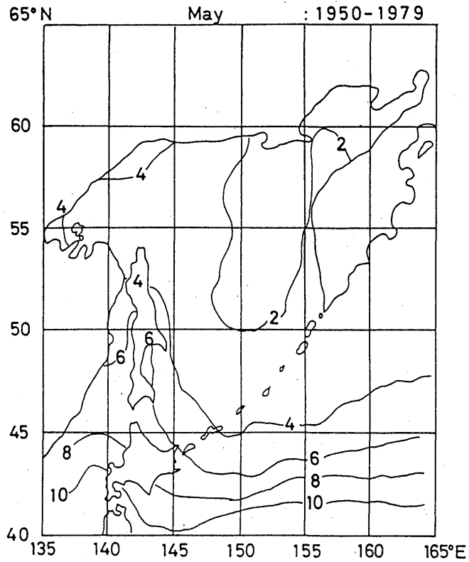
Fig. 4. 3 Monthly mean surface air temperature (°C) (May-June)
