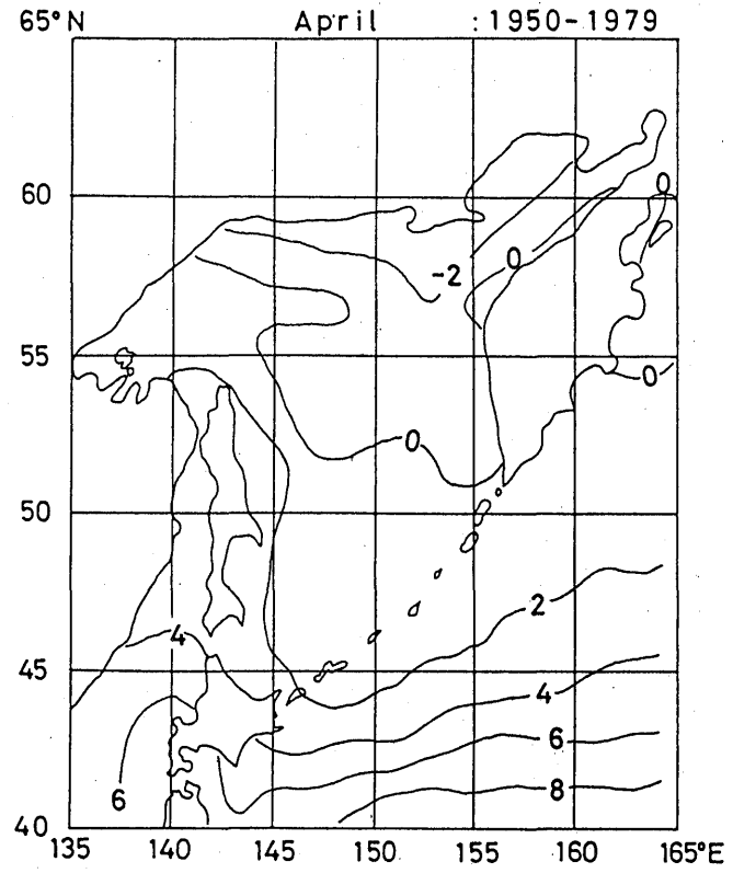
Fig. 4. 2 Monthly mean surface air temperature (°C) (March-April)
