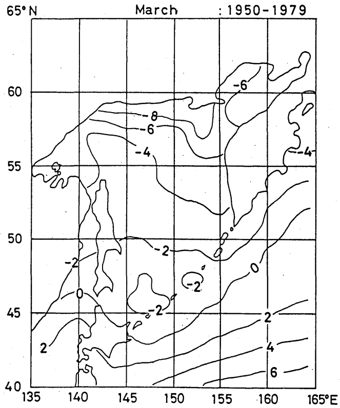
Fig. 4. 2 Monthly mean surface air temperature (°C) (March-April)
