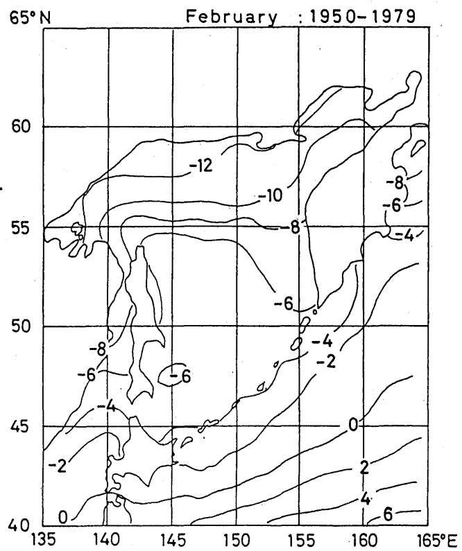
Fig. 4. 1 Monthly mean surface air temperature (°C) (January-February)
