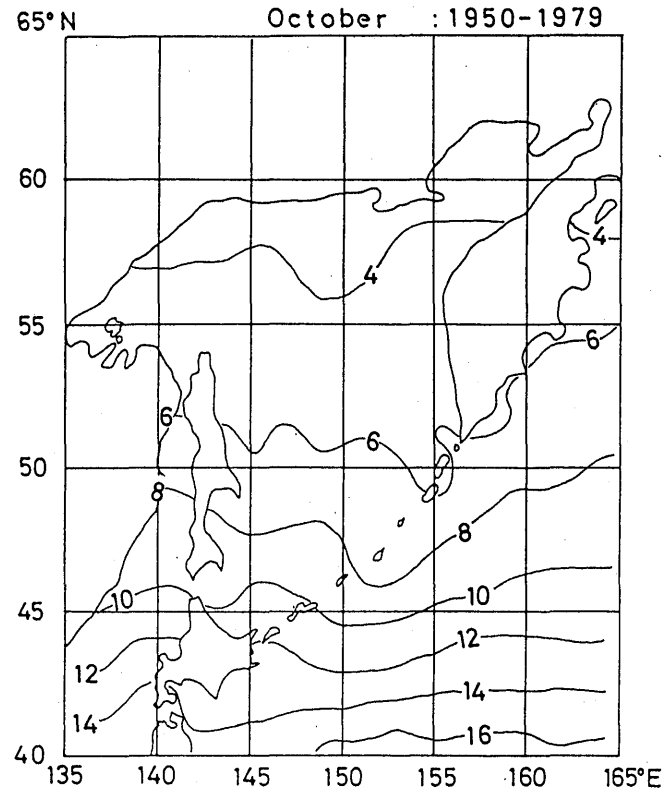
Fig. 4.5 Monthly mean surface air temperature (°C) (September–October)
