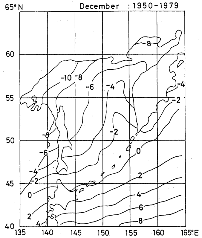
Fig. 4. 6 Monthly mean surface air temperature (°C) (November-December)
