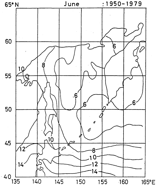
Fig. 4. 3 Monthly mean surface air temperature (°C) (May-June)
