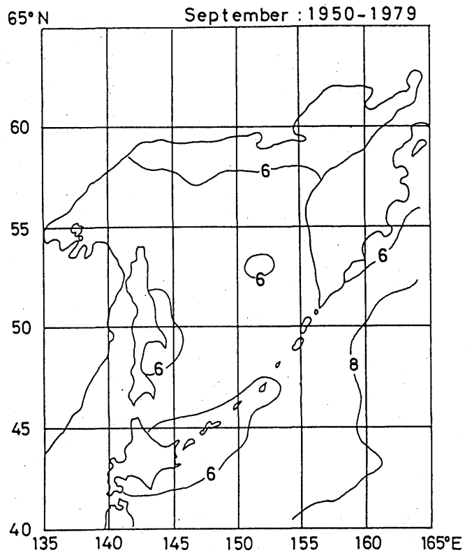
Fig. 2. 5 Monthly mean wind speed (m/s) (September-October)
