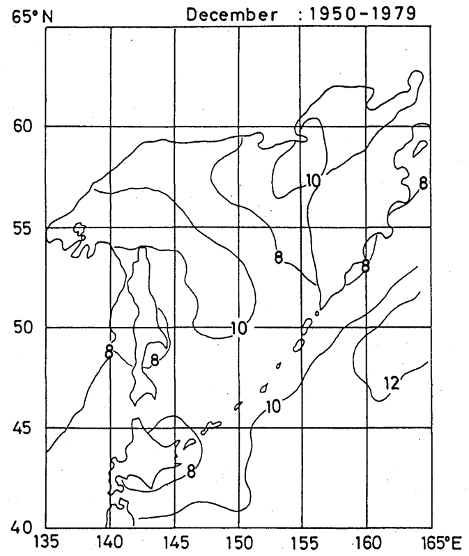
Fig. 2.6 Monthly mean wind speed (m/s) (November-December)
