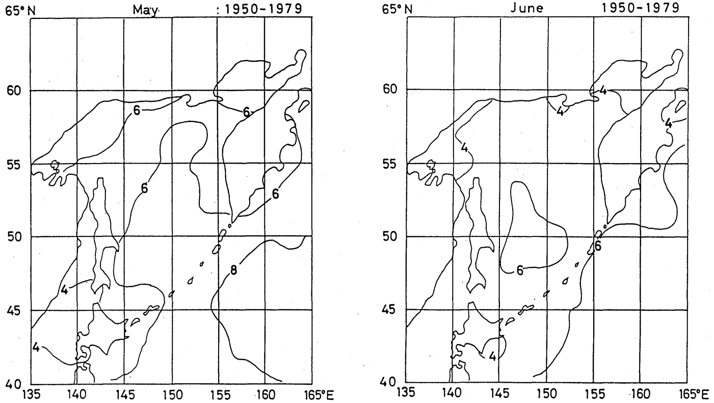
Fig. 2. 3 Monthly mean wind speed (m/s) (May-June)
