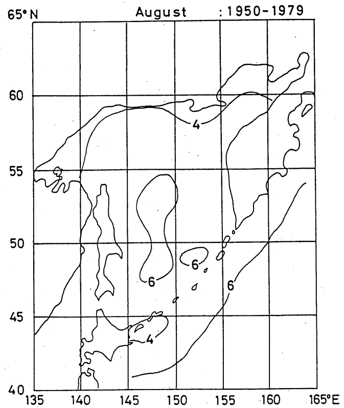
Fig. 2. 4 Monthly mean wind speed (m/s) (July-August)
