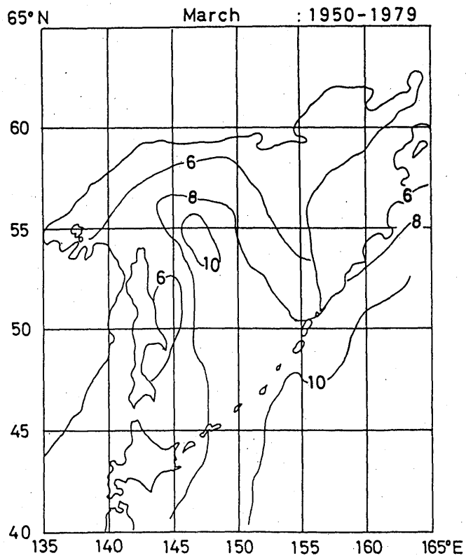
Fig. 2. 2 Monthly mean wind speed (m/s) (March-April)
