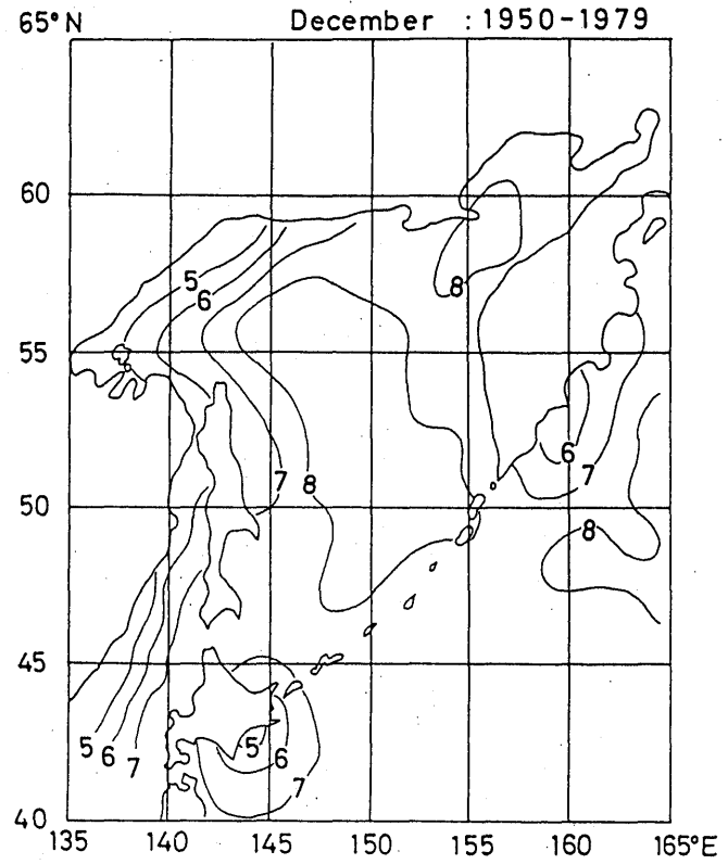
Fig. 6. 6 Monthly mean cloud amount (0-10) (November-December)
