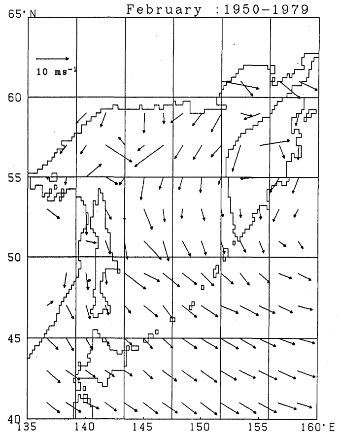
Fig. 3. 1 Monthly mean wind vector (January-February)
