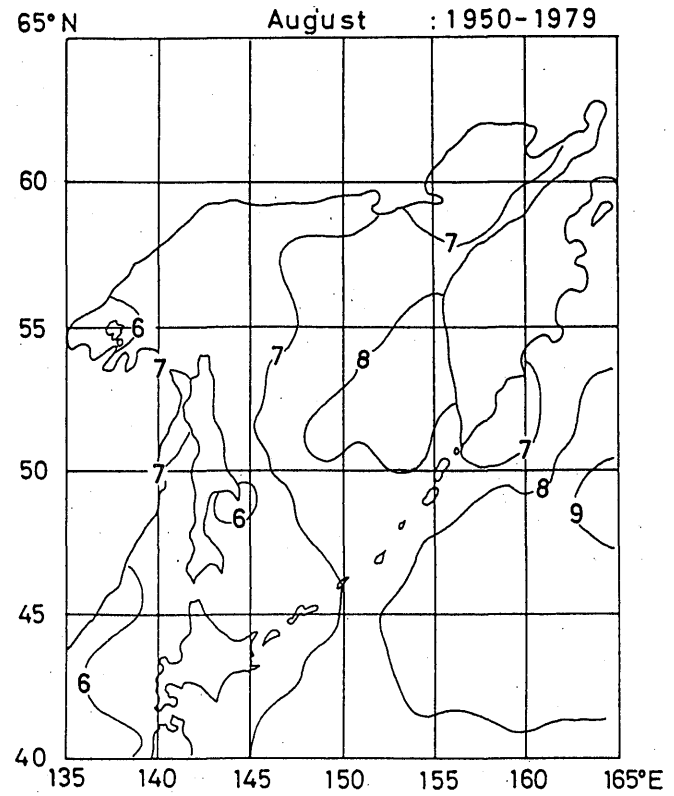
Fig. 6. 4 Monthly mean cloud amount (0-10) (July-August)
