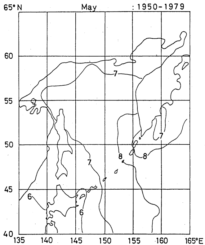
Fig. 6. 3 Monthly mean cloud amount (0-10) (May-June)
