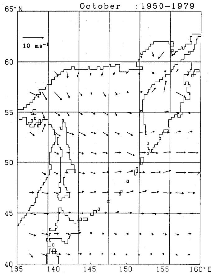
Fig. 3. 5 Monthly mean wind vector (September-October)
