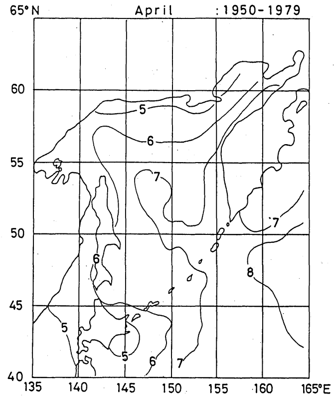
Fig. 6. 2 Monthly mean cloud amount (0-10) (March-April)
