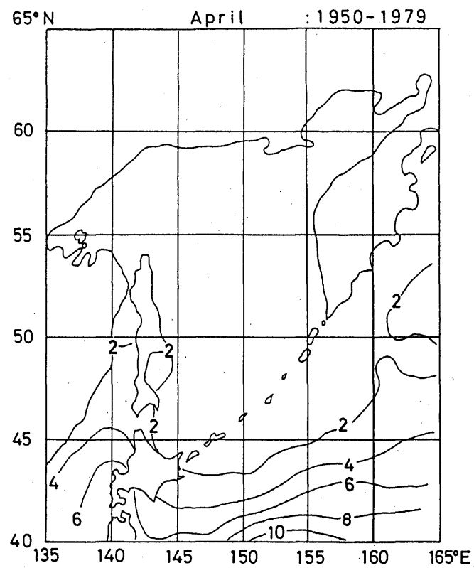
Fig. 5. 2 Monthly mean sea surface temperature (°C) (March-April)
