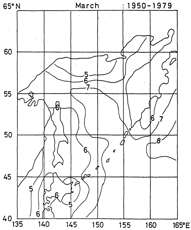
Fig. 6. 2 Monthly mean cloud amount (0-10) (March-April)
