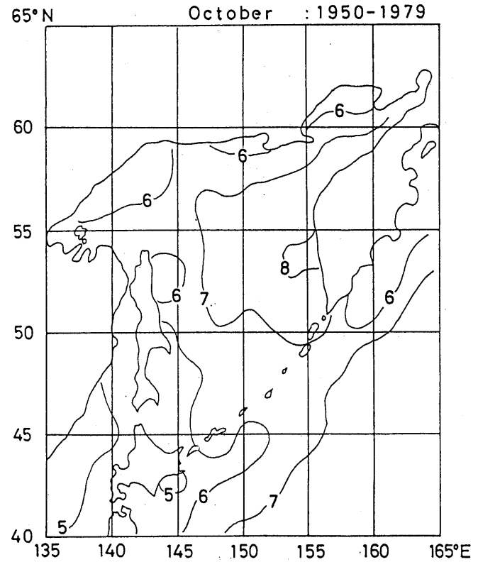
Fig. 6. 5 Monthly mean cloud amount (0-10) (September-October)
