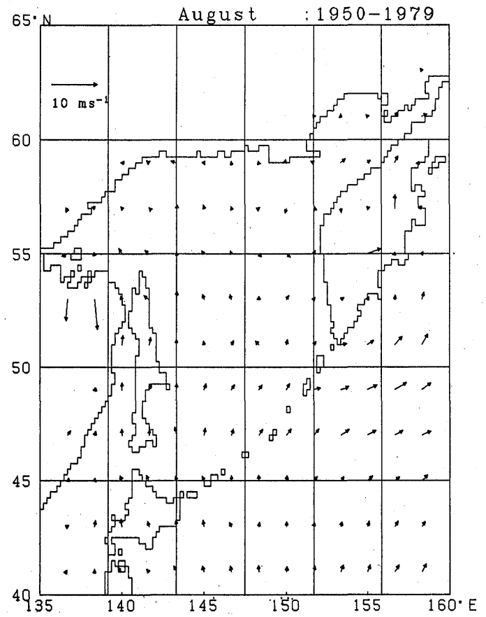
Fig. 3. 4 Monthly mean wind vector (July-August)
