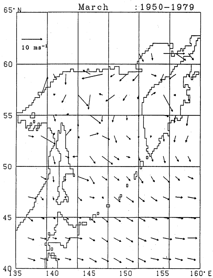
Fig. 3.2 Monthly mean wind vector (March-April)
