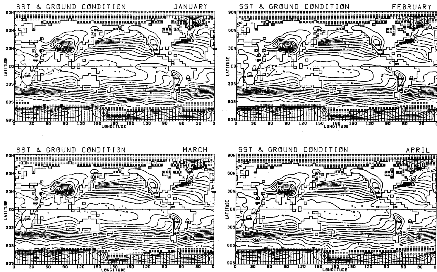
Fig. 0.1 . Topography used in the MRI-GCM-I. Contour interval is 500 m. The sea surface temperature distributions are shown over the ocean, together with land ice distributions indicated with "I", and sea ice distributions indicated with "=" for January, February, March and April. Contour interval for sea surface temperature is 2°C. The grid points indicated with "L" are lake points.
