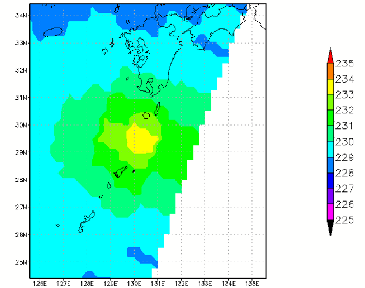
AMSU Limb corrected CH07 of T0423 at 2004-10-19 18:45:00Z
