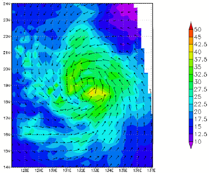
QSV3 of T0423 at 2004-10-16 21:12:00Z
