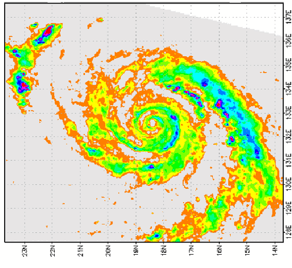
AMSR-E PCT85 of T0423 at 2004-10-16 17:04:00Z
