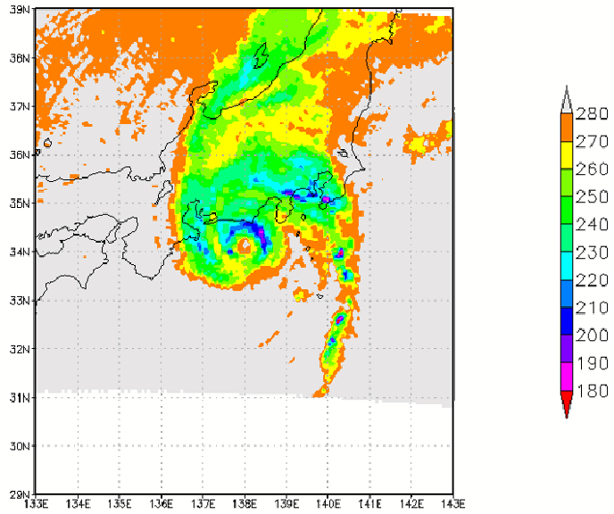
TMI PCT85 of T0422 at 2004-10-09 05:16:00Z
