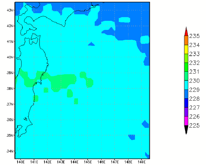
AMSU Limb corrected CH07 of T0422 at 2004-10-09 17:15:00Z
