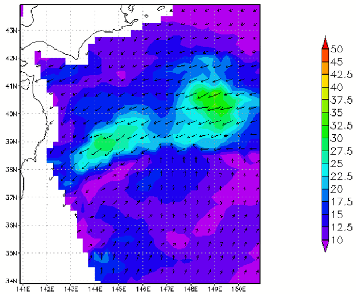
QSV3 of T0422 at 2004-10-09 19:18:00Z
