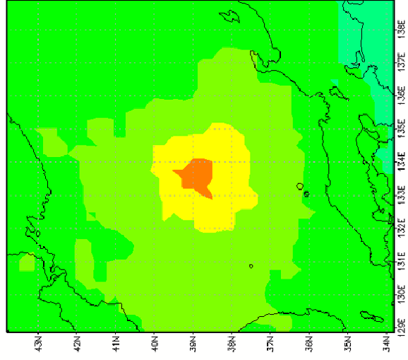
AMSU Limb corrected CH07 of T0415 at 2004-08-19 09:25:00Z
