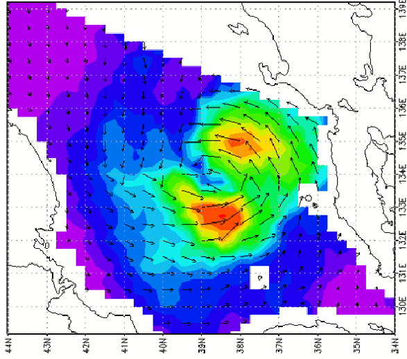
QSV3 of T0415 at 2004-08-19 09:59:00Z
