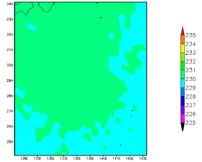
AMSU Limb corrected CH07 of T0411 at 2004-08-03 21:22:00Z
