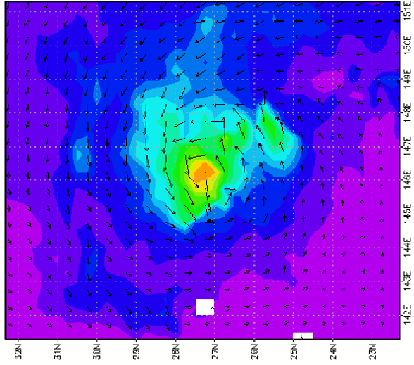
QSV3 of T0410 at 2004-07-26 19:54:00Z
