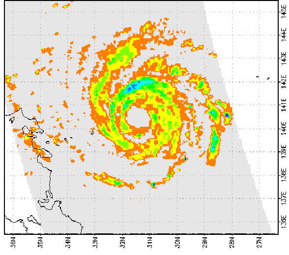
TMI PCI85 of T0410 at 2004-07-28 15:49:00Z
