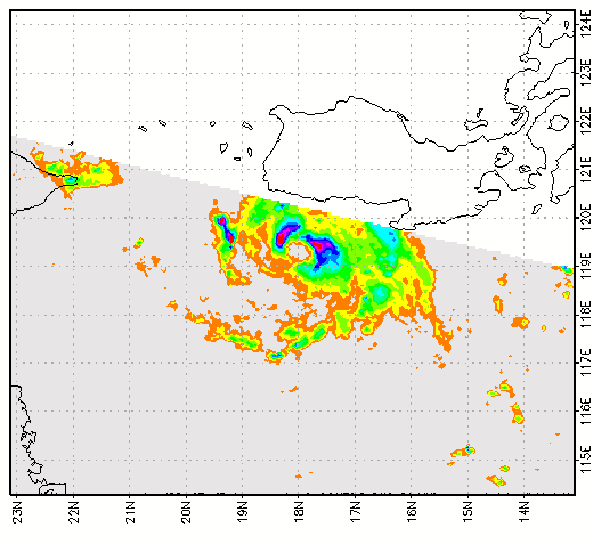
AMSR-E PCT85 of T0404 at 2004-06-07 18:12:00Z
