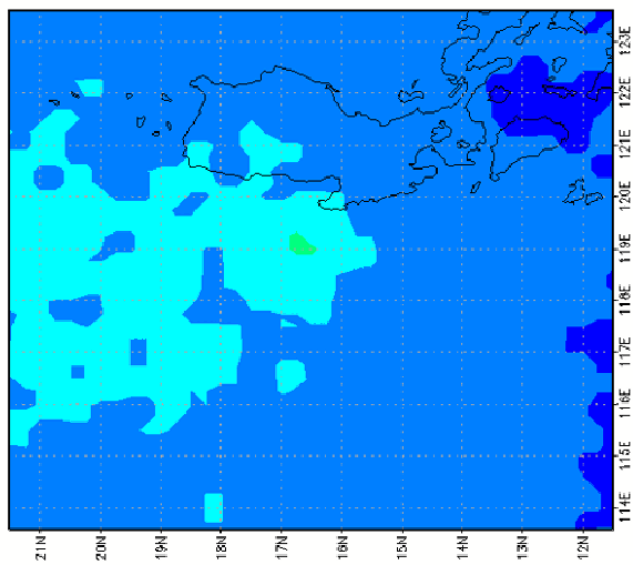
AMSU Limb corrected CH07 of T0404 at 2004-06-06 22:37:00Z
