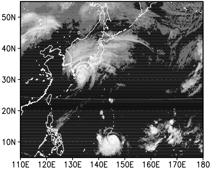
GOES-9 IR1
