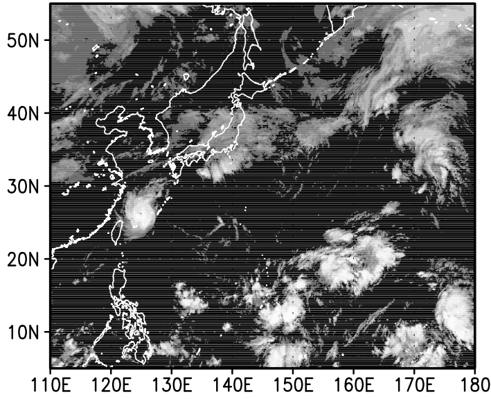
GOES-9 IR1
