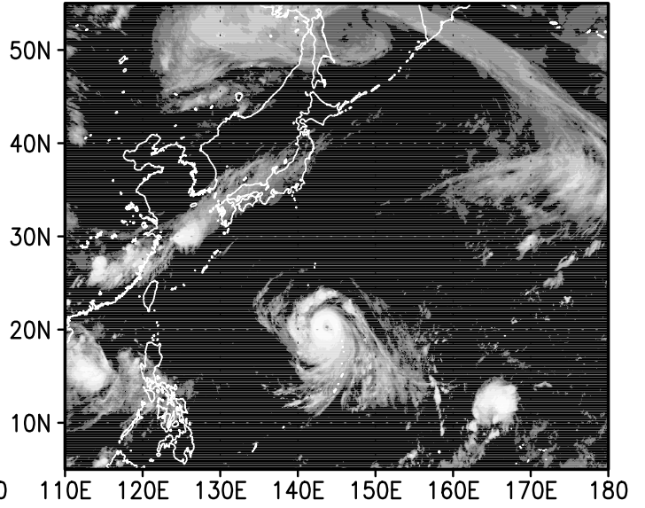
12z02sep2004
