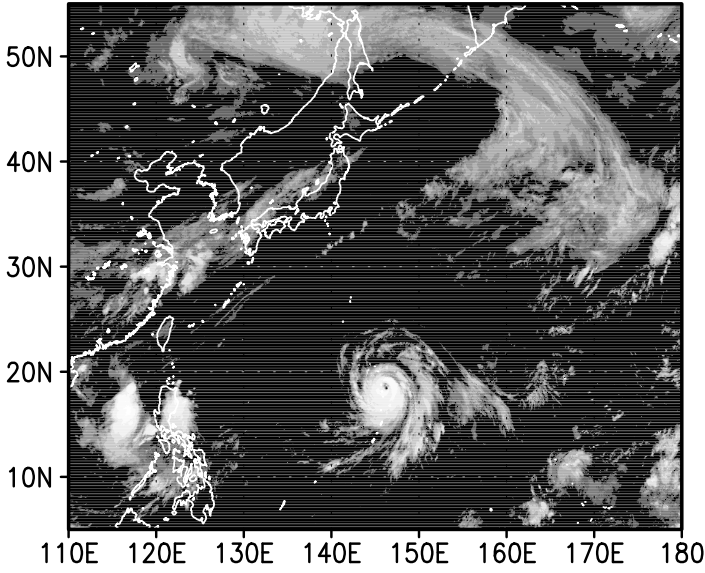
00z02sep2004
