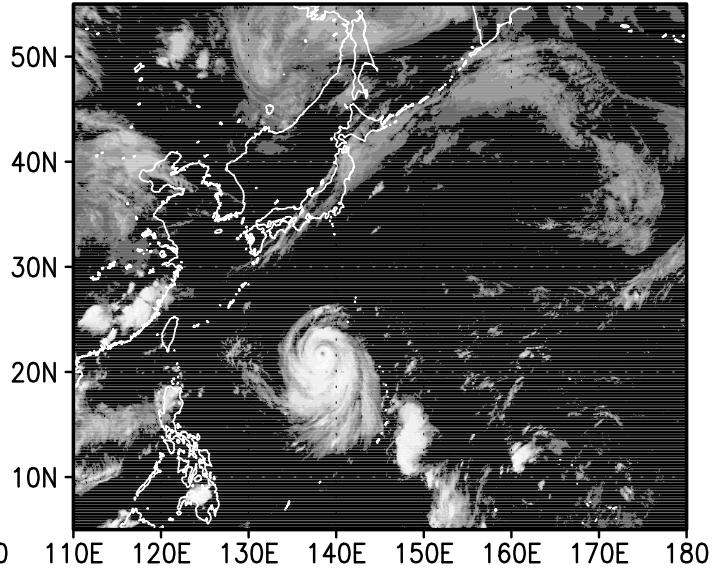
12z03sep2004
