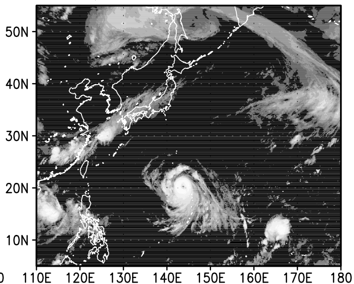
12z01sep2004
