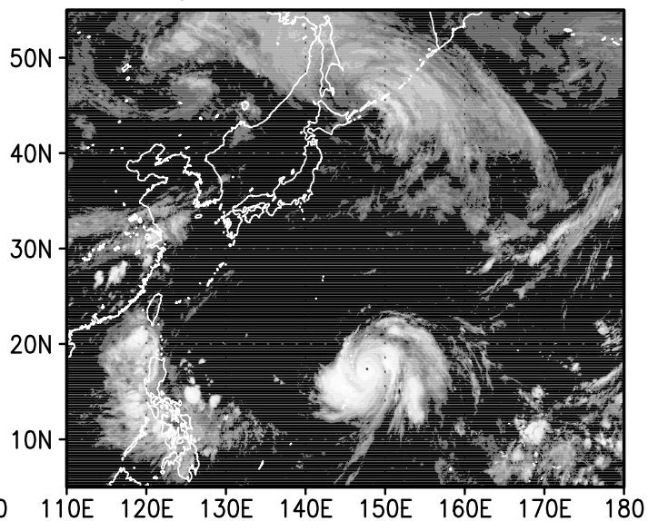
12z01sep2004
