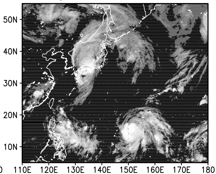
12z31aug2004
