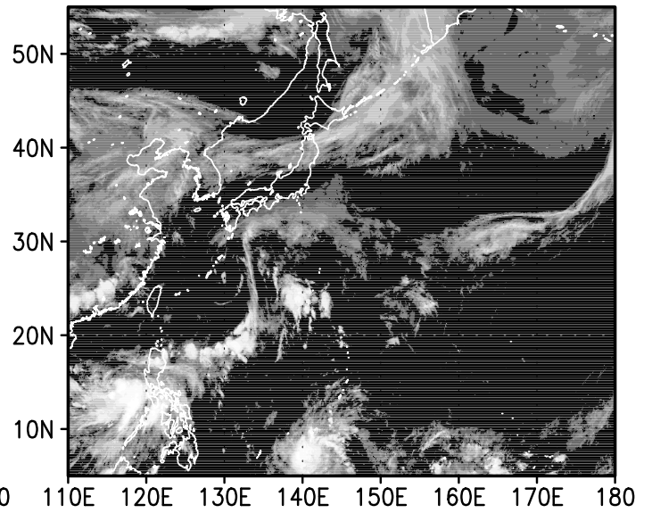
12z06jun2004
