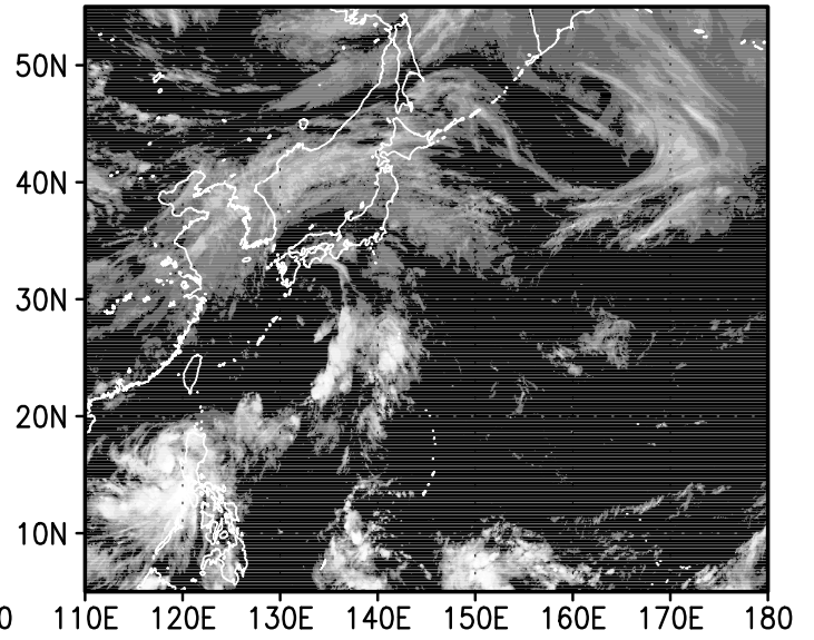
12z07jun2004
