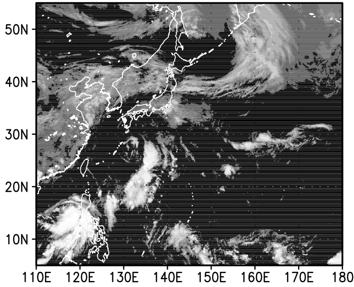
00z07jun2004
