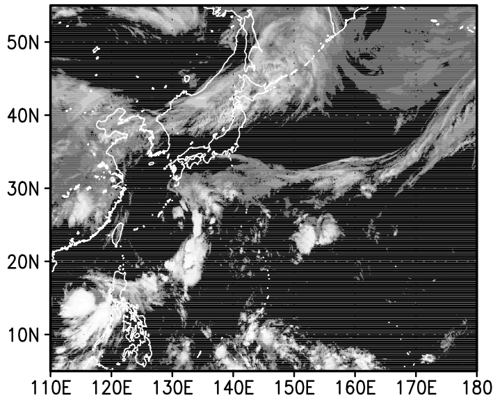
00z06jun2004
