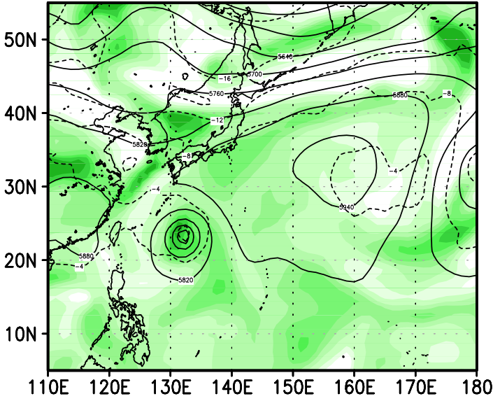
00z05sep2004
