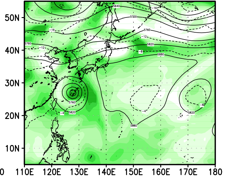
12z06sep2004
