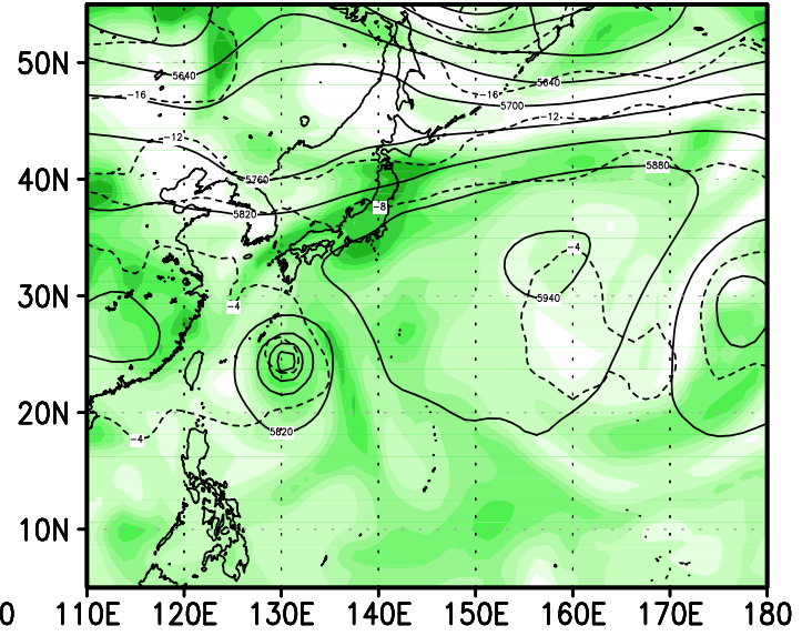
12z05sep2004
