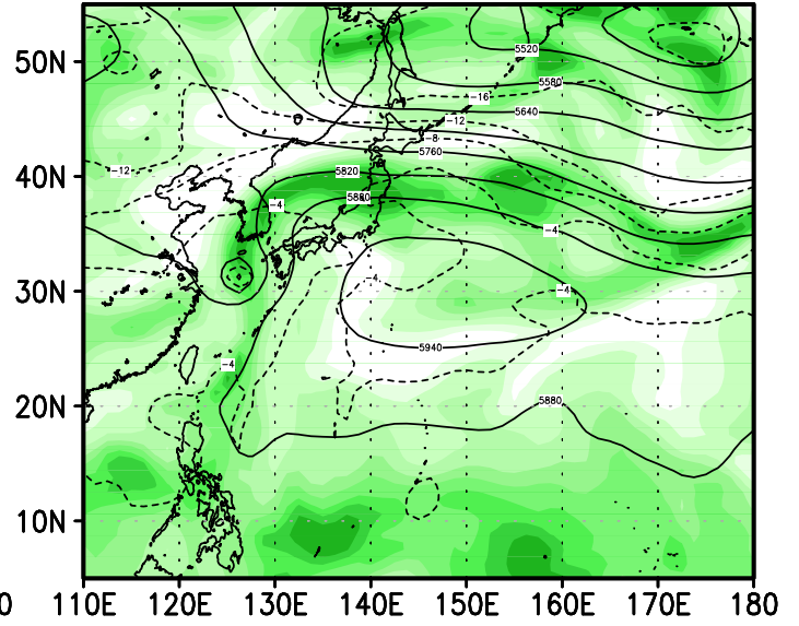
12z19aug2004
