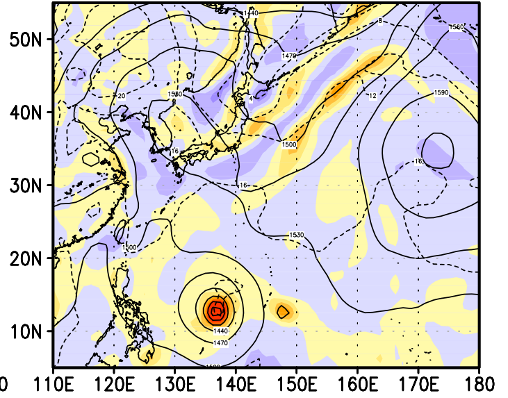
12z16jun2004
