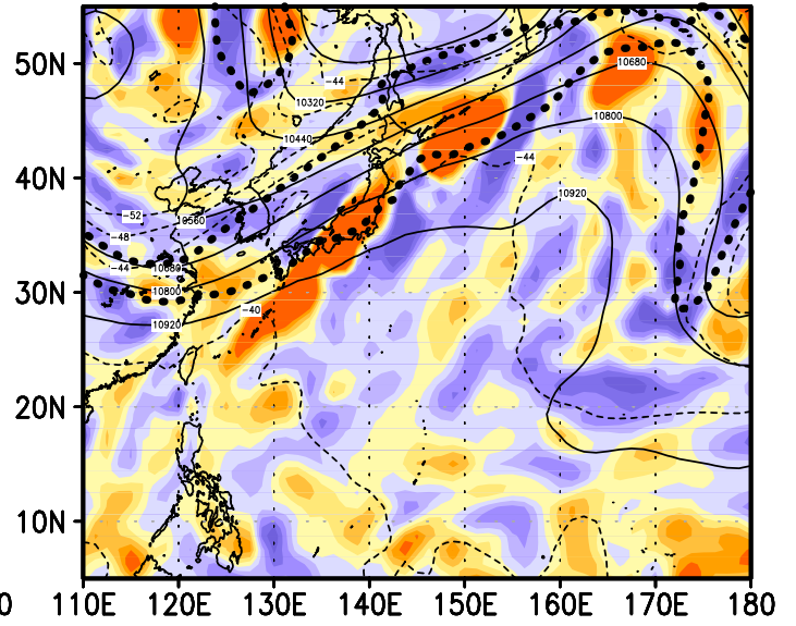
12z09jun2004
