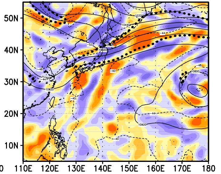
12z10jun2004
